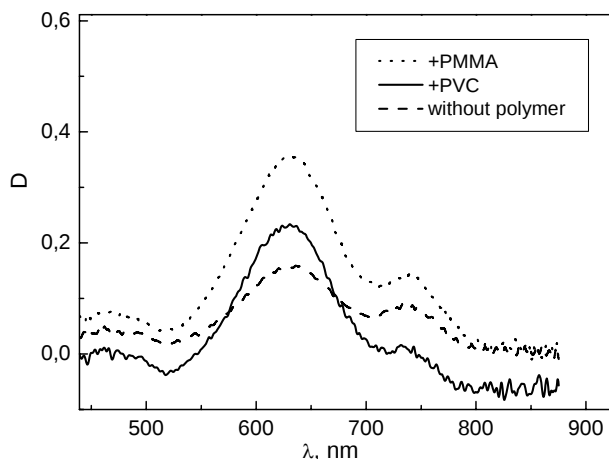
Fig. 5. Absorption spectra of 2 at U = 2 V in two electrode cell in acetonitrile solution (0.05 M \text{LiClO}_4 ), PMMA (20 mg/ml) acetonitrile solution (0.05 M \text{LiClO}_4 ), PVCa (20 mg/ml) acetonitrile solution (0.05 M \text{LiClO}_4 ). The concentration of 2 is 1 mg/ml
