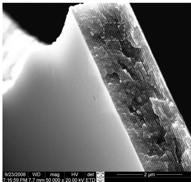
Fig. 1. SEM image of Cu/Cr multilayer film cross-section with magnification 50 000
