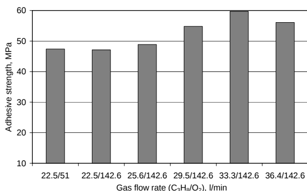
Fig. 7. Dependence of WC-12%Co coating, sprayed by MicroJet gun, adhesive strength on gas flow rate
