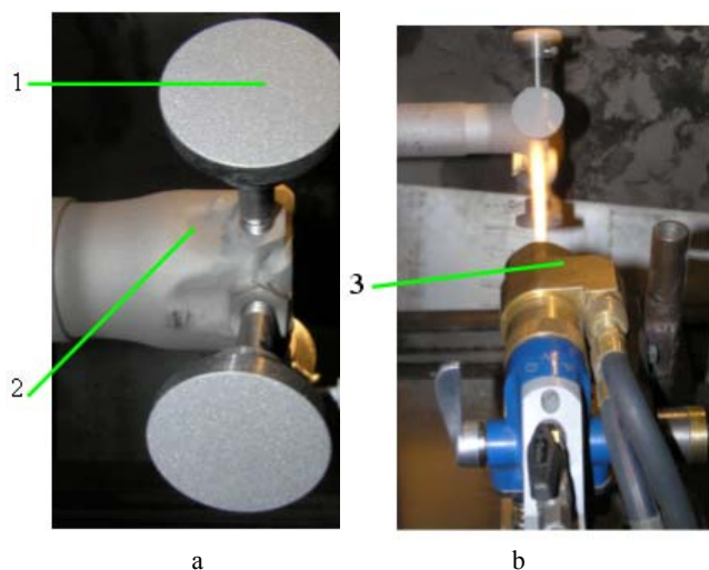
Fig. 3. Deposition of WC-12%Co coating on the specimens for determining adhesive strength: 1 – specimen; 2 – rotation device; 3 – spraying gun
