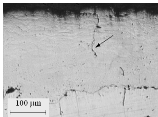
Fig. 4. Microstructure of the WC-12%Co coating sprayed by MicroJet gun at 36.4 l/min fuel gas supply rate
