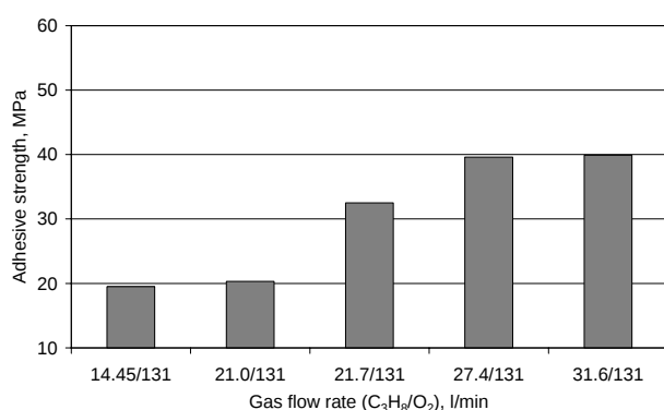
Fig. 8. Dependence of WC-12%Co coating, sprayed by modified TopJet/2 gun, adhesive strength on gas flow rate
