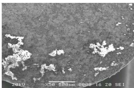
Fig. 9. The specimen's surface after coating was separated from substrate
