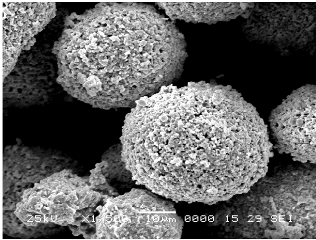
Fig. 1. Microstructure of WC-12%Co powder
