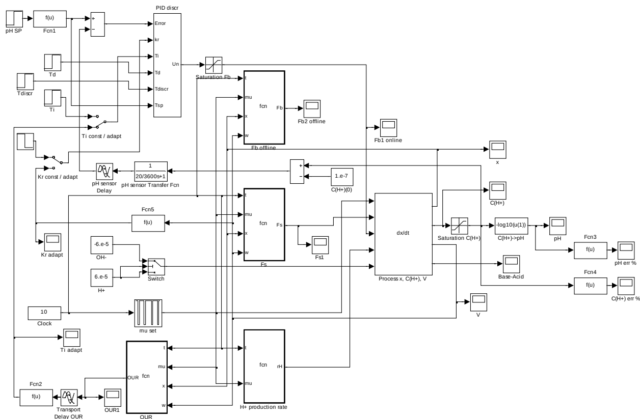
Figure 5. General view of the adaptive pH control system model
