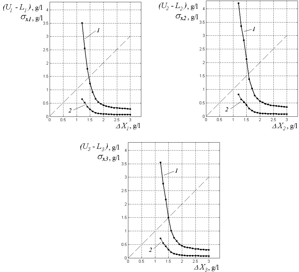
Figure 4. Relationships between the ranges of factor variation \Delta X_i and the 95 % confidence interval U_i - L_i (1) and standard deviation \sigma_{xi} (2) of the optimal point estimations
