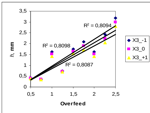
Fig. 8. Dependence of the height of the effects ( h ), mm upon the overfeed ( \eta )
