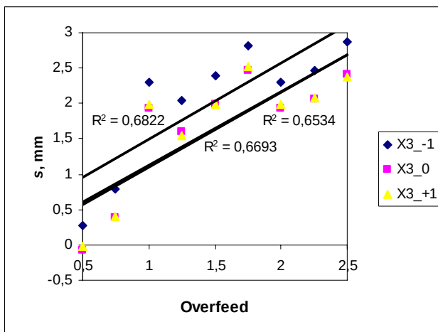
Fig. 9. Dependence of the width of the effects ( s ), mm upon the overfeed ( \eta )
