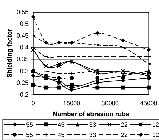
Fig. 10. Shielding factor of PES/cotton fabrics versus the number of abrasion rubs ( — fabrics with S-Shield PES yarns; — — fabrics with Silverflex-170 yarns) (the legend shows the number of weft yarns between conductive ones)
