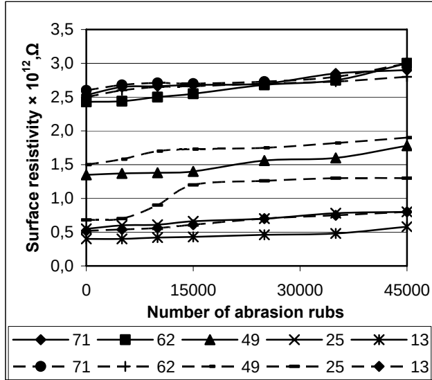
Fig. 1. Surface resistivity of PES fabrics versus the number of abrasion rubs ( — fabrics with S-Shield PES yarns; - - - fabrics with Silverflex-170 yarns) (the legend shows the number of weft yarns between conductive ones)
