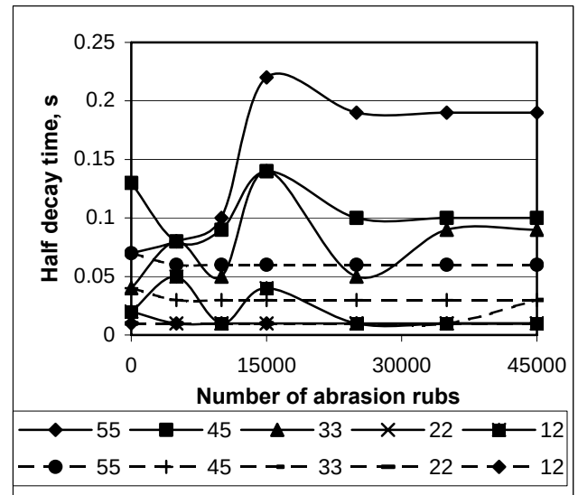
Fig. 11. Half decay time of PES/cotton fabrics versus the number of abrasion rubs ( — fabrics with S-Shield PES yarns; — — fabrics with Silverflex-170 yarns) (the legend shows the number of weft yarns between conductive ones)
