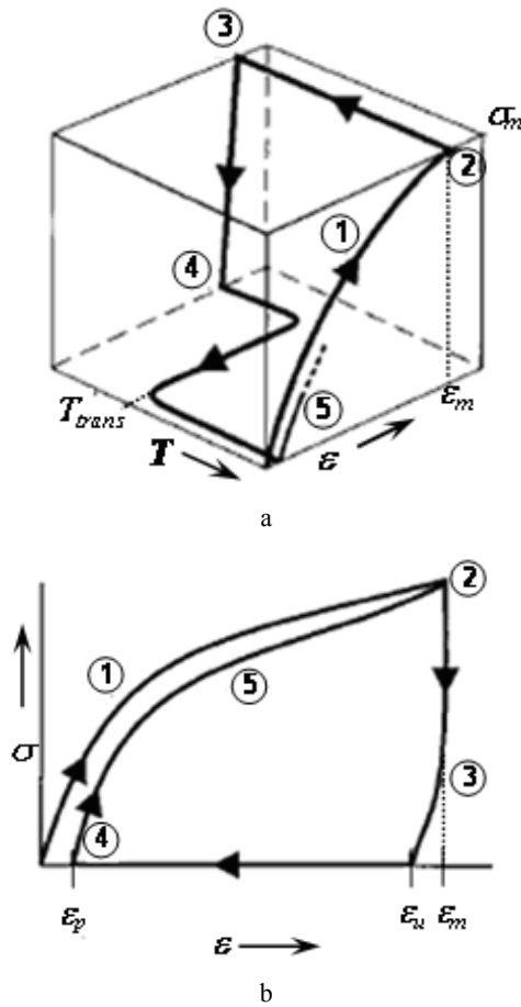
Fig. 2. Cyclic tensile testing path (a) and schematic stress-strain curves (b) under drawing at high temperature and thermal recovery
