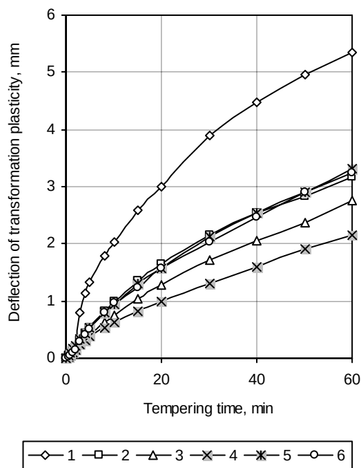
Fig. 2. Influence of ageing on transformation plasticity of steel 20X13 during bending at 650 °C (1 h, 90 MPa). Duration of ageing (h): 1 – 0; 2 – 1; 3 – 2; 4 – 5; 5 – 10; 6 – 48
