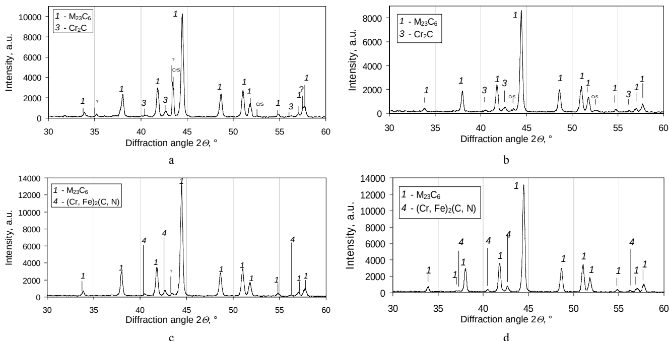
Fig. 5. X-ray diffraction patterns of 20X13 steel bent at 650 °C: a – after hardening; b – after hardening and 1 h ageing; c – after hardening and 10 h ageing; d – after hardening and 48 h ageing.
