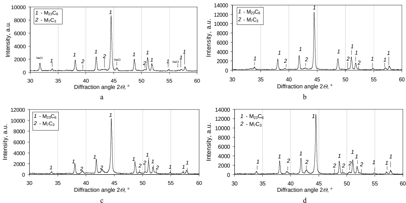
Fig. 4. X-ray diffraction patterns of 20X13 steel bent at 520 °C: a – after hardening; b – after hardening and 1 h ageing; c – after hardening and 10 h ageing; d – after hardening and 48 h ageing.
