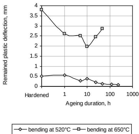
Fig. 3. Influence of ageing on plastic deformation of steel 20X13 during bending
