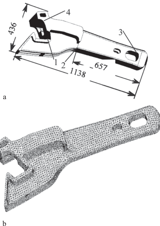
Fig. 2. The body of the automatic coupler in railway carriages (a); 3D FEM mesh for the automatic coupler (b)
