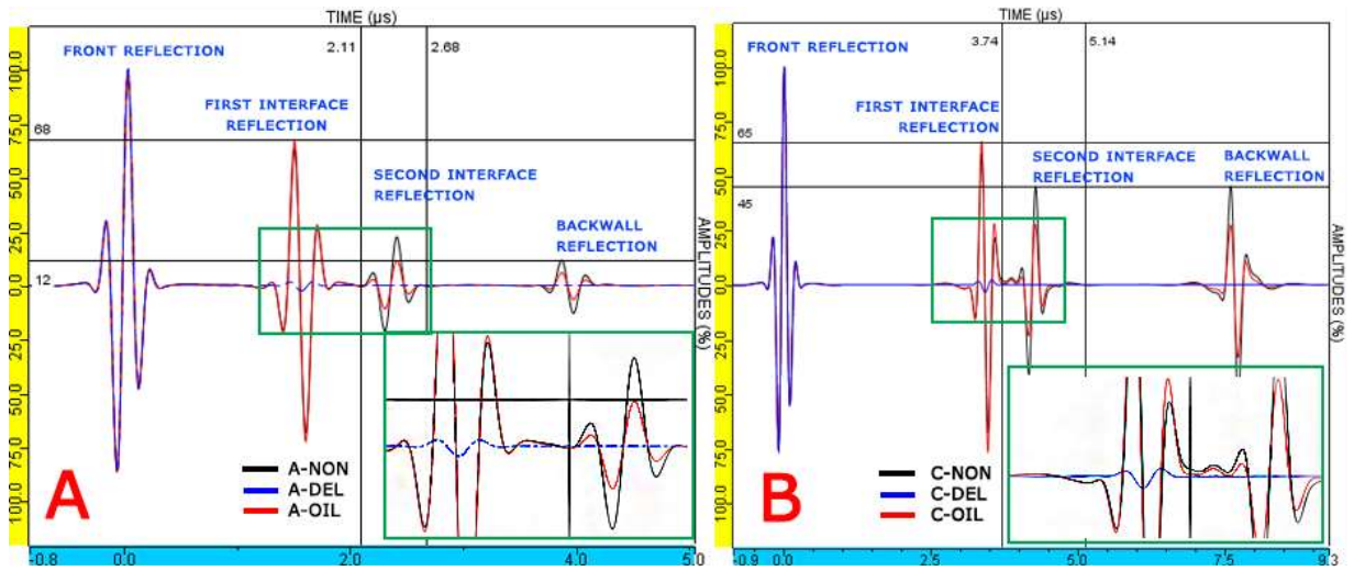
Figure 2. A-Scan results of six different cases calculated by CIVA 2017.
