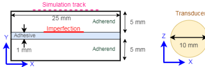
Figure 1. Schematic representation of the model (on the left) with the dimensions. Imperfection stands for delamination or oil-contamination. Transducer size and shape (on the right).
