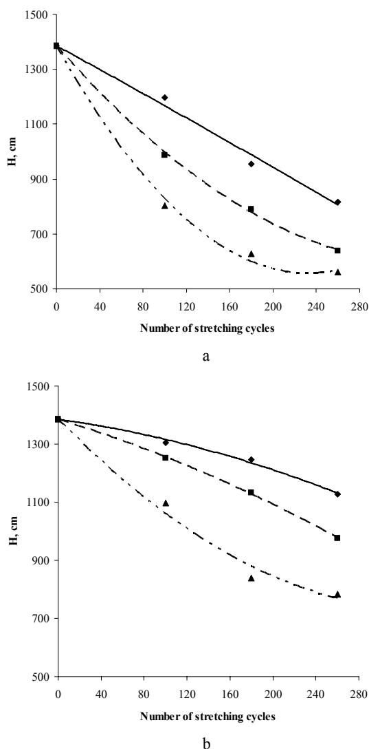
Fig. 4. The dependence of resistance to water penetration on number of stretching cycles at warp direction (a) and weft direction (b) of sample B: ◆ and — 15 % fixed elongation, ■ and — 20 % fixed elongation, ▲ and — 25 % fixed elongation
