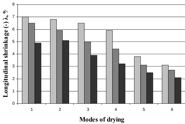
Fig. 4. The dependence of shrinkage in longitudinal direction \lambda of I1 fabric (dried in different conditions) upon the number of washing and drying cycles (marked as in Fig. 3)
