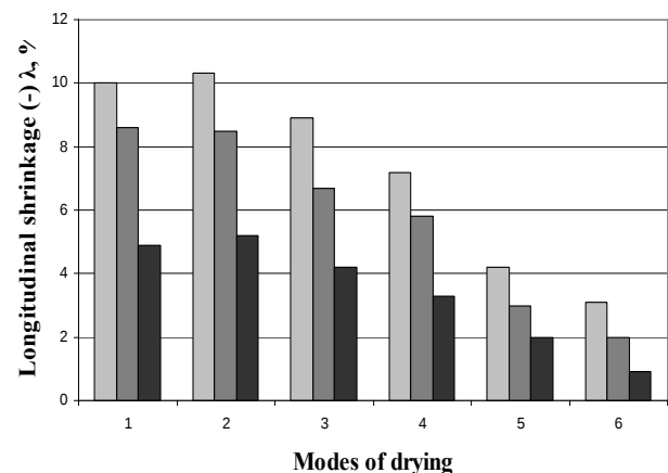
Fig. 3. The dependence of shrinkage in longitudinal direction \lambda of PJ fabric (dried in different conditions) upon the number of washing and drying cycles: □ – shrinkage value after the first cycle, ▤ – shrinkage value after the second cycle, ■ – shrinkage value after the third cycle; (1 – hanged on a line in course direction, 2 – hanged on a line in wale direction, 3 – spread on a smooth surface, 4 – spread on a heated surface, 5 – winded by hot air, 6 – in a tumble-dryer)
