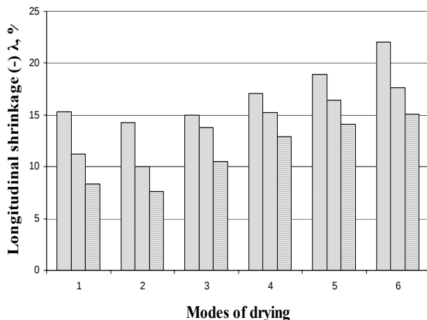
Fig. 1. The dependence of shrinkage in longitudinal direction \lambda of PJ – ▨, II – ▩, and I2 – ▤ fabrics upon the mode of drying: 1 – hanged on a line in course direction, 2 – hanged on a line in wale direction, 3 – spread on a smooth surface, 4 – spread on a heated surface, 5 – winded by hot air, 6 – in a tumble-dryer
