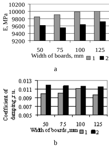
Fig. 3. Variation of modulus of elasticity (a) and coefficient of damping (b) of the boards with radial cut and scantlings forming them: 1 – parameters of uncut boards; 2 – average parameters of scantlings forming some parts of boards
