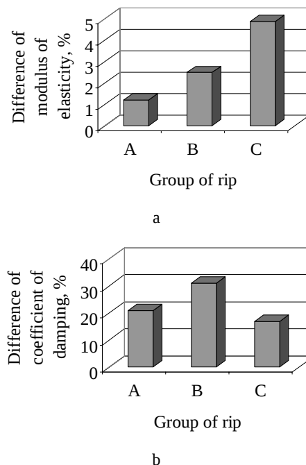
Fig. 6. Values of average differences of modulus of elasticity (a) and coefficient of damping (b) of the boards with radial and combined cuts and their scantlings
