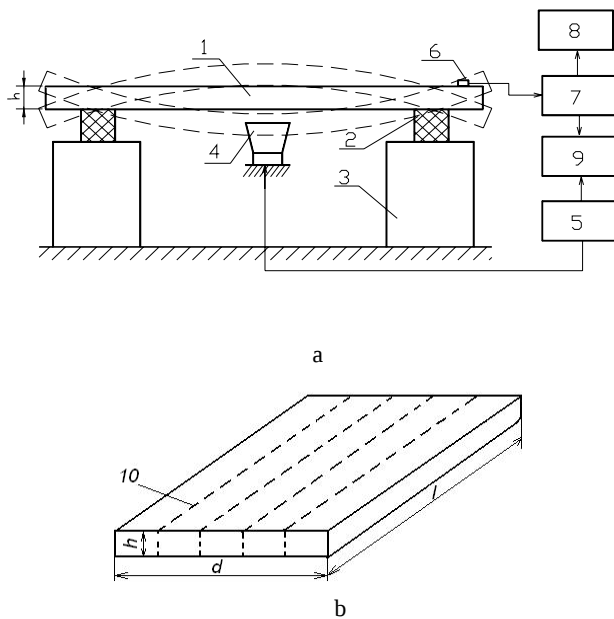
Fig. 2. Schemes of a test stand for wood articles (a) and of board (b): 1 – wood assortment and type of its inflection (mode); 2 – elastic elements; 3 – massive support; 4 – acoustic vibrator; 5 – generator; 6 – vibrosensor; 7 – gauge; 8 – oscilloscope; 9 – phasometer; 10 – location of a rip; l – length of a board, d – width, h – thickness
