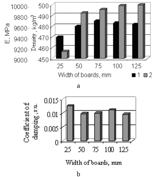
Fig. 5. Variation regularities of average density (a, 1), modulus of elasticity (a, 2) and coefficient of damping (b) of the boards with radial cut
