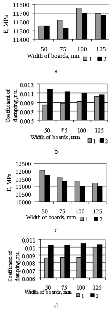
Fig. 4. Variation of modulus of elasticity and coefficient of damping of the boards with tangential cut (a, b) and combined (c, d) cut and their scantlings; where 1 – parameters of uncut board; 2 – average parameters of scantlings forming a respective part of a sample
