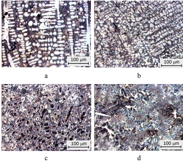
Fig. 7. Microstructures of the layers obtained in overlay welding of Cr3 steel by Cb 08 wire under the AMS1 flux containing 52 % WC-8 % Co and SB-5 powder in the allowing amount, %: a-0, b-3, c-6, d-10
