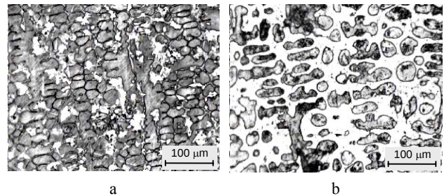
Fig. 9. Microstructures of the layers produced by overlay welding of Cr3 steel with Cb 08 wire under the AMS1 flux containing 29 % WC-8 % Co, 6 % graphite and varying amount of Fe-70 % Mn powder: a-0 %, b-10 %
