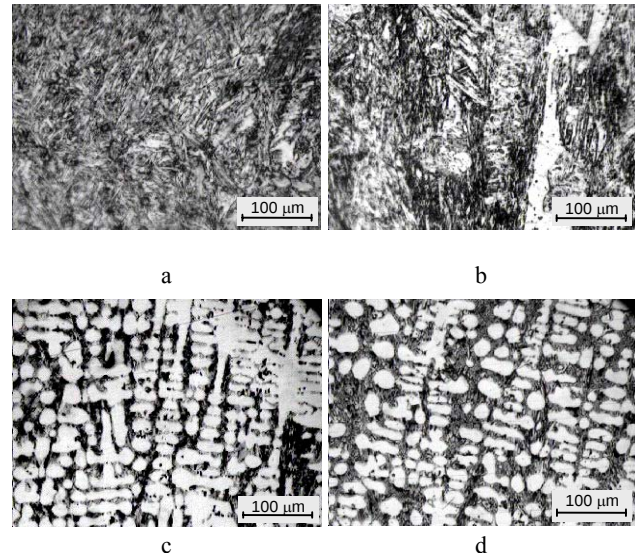
Fig. 1. Microstructures of layers obtained in overlay welding of Cr3 steel by Cb 08 wire under the AMS1 flux containing 11 % graphite (a), 25 % chromium (b), 6.5 % graphite and 26.5 % chromium (c), 10 % graphite and 25.5 % chromium powder (d)
