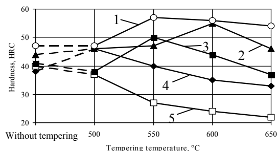
Fig. 2. Dependence of layers hardness on tempering temperature of Cr3 steel subjected to overlay welding with Cb 08 wire under the AMS1 flux mixed with graphite and chromium powder
