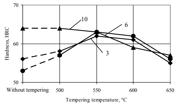
Fig. 6. Dependence of layers hardness on tempering temperature of Cr3 steel subjected to overlay welding by Cв 08 wire under the AMS1 flux mixed with WC-8 % Co (52 %) and SB-5 (3, 6 and 10 %) powder. Numbers at the curves show percentage amount of SB-5 powder in the flux
