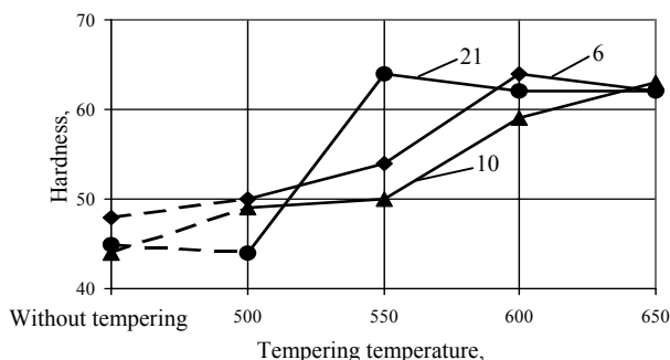
Fig. 8. Dependence of layers hardness on tempering temperature of Cr3 steel overlayed by Cb 08 wire under the AMS1 flux mixed with graphite (6 %), WC-8 % Co (29 %) and Fe-70 % Mn powder. Numbers at the curves show percentage amount of Fe-70 % Mn powder in the flux
