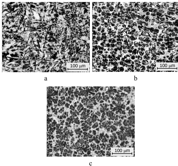
Fig. 4. Microstructures of layers obtained in overlay welding of Cr3 steel by Cв 08 wire under the AMS1 flux containing 10 % graphite, 10 % chromium, 16 % molybdenum and varying amount of SiCaBa powder: a – 10 %, b – 15 %, c – 21 %
