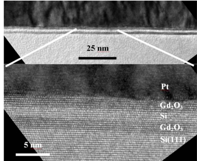
Fig. 1. HRTEM micrographs of \text{Gd}_2\text{O}_3/\text{Si}/\text{Gd}_2\text{O}_3 double barrier structure grown on Si(111) by solid-phase-epitaxy [7]
