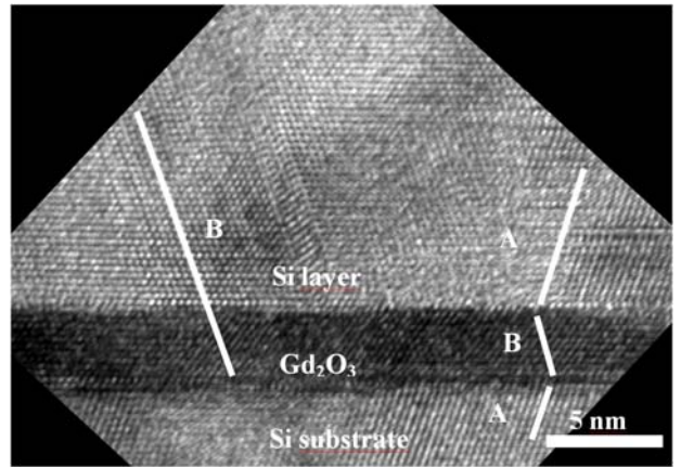
Fig. 12. Cross-sectional low (a) and high (b), (c) magnification TEM micrographs of Si (111)/ \text{Gd}_2\text{O}_3 /Si structure. The Si layer was grown by vapour phase epitaxy on single oriented crystalline Si islands
