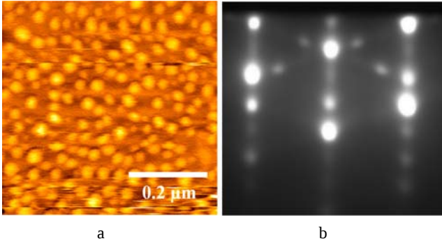
Fig. 8. AFM picture (a) and RHEED pattern (b) of Si islands grown on \text{Gd}_2\text{O}_3 [10]
