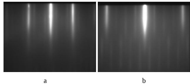
Fig. 2. Typical RHEED patterns of 4 nm \text{Gd}_2\text{O}_3 grown on Si(111) obtained in (a) \langle 110 \rangle and (b) \langle 112 \rangle azimuth
