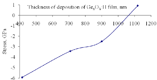
Fig. 7. Residual stress of \text{Ge}_x\text{O}_y\text{:H} films as a function of the film thickness
