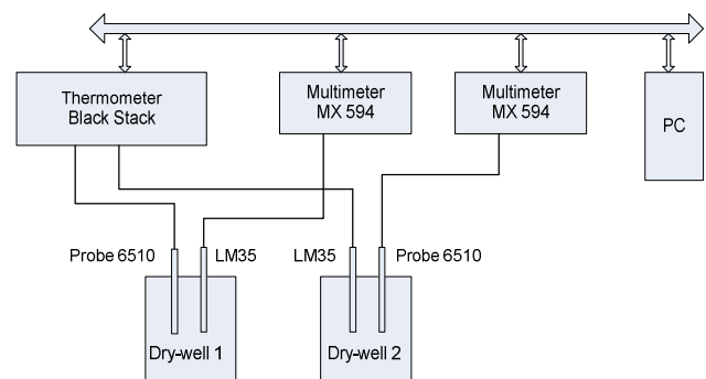
Fig. 1. The structure of measurement equipment
