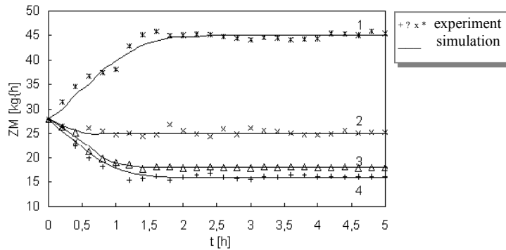
Figure 5. Volume of inlet air (ZM) over time to reach the setpoint x_{50} : comparison of real process with the simulated control system; (1) x_{50} = 370\mu\text{m} , (2) x_{50} = 400\mu\text{m} , (3) x_{50} = 420\mu\text{m} , (4) x_{50} = 430\mu\text{m}
