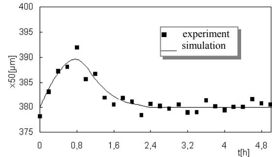
Figure 8. Changes in x_{50} following an initial increase in the volume of the water feed (WP) from 13.5 to 15 ml/min
