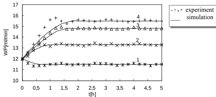
Figure 6. Volume of water feed (WP) over time required to reach the setpoint x_{50} : comparison of real process with the simulated control system; (1) x_{50} = 370\mu\text{m} , (2) x_{50} = 400\mu\text{m} , (3) x_{50} = 420\mu\text{m} , (4) x_{50} = 430\mu\text{m}
