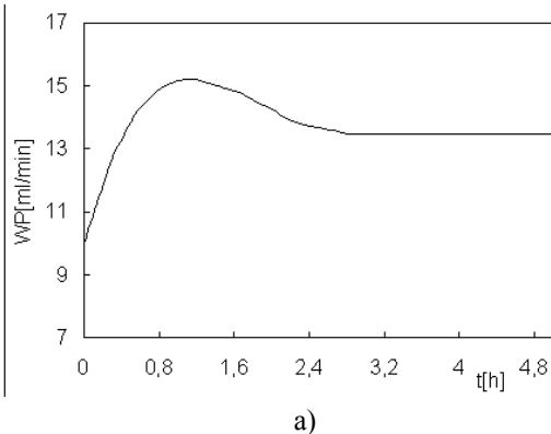
Figure 9. a) change in volume of solid over time following an initial increase in the volume of inlet air; b) change in volume of water feed over time following an initial increase in the volume of inlet air
