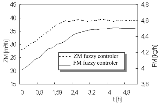
Figure 7. Changes in volume of inlet air (ZM) and volume of solid material (FM) following an initial jump in the water feed volume
