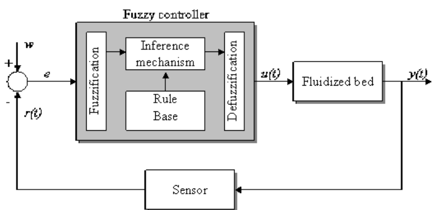
Figure 2. Fuzzy closed-loop control system. w – setpoint, e – error, r(t) – measured value, u(t) – control action, y(t) – process output
