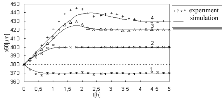
Figure 4. x_{50} over time for different setpoint defaults: comparison of real process with simulated control system; (1) x_{50} = 370\mu\text{m} , (2) x_{50} = 400\mu\text{m} , (3) x_{50} = 420\mu\text{m} , (4) x_{50} = 430\mu\text{m}
