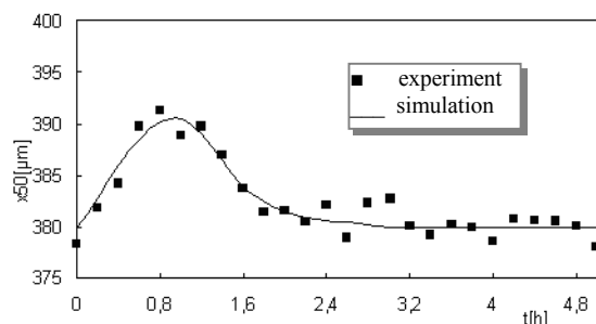
Figure 10. Change in x_{50} following an initial increase in the volume of inlet air: comparison of experiment with model-related simulation
