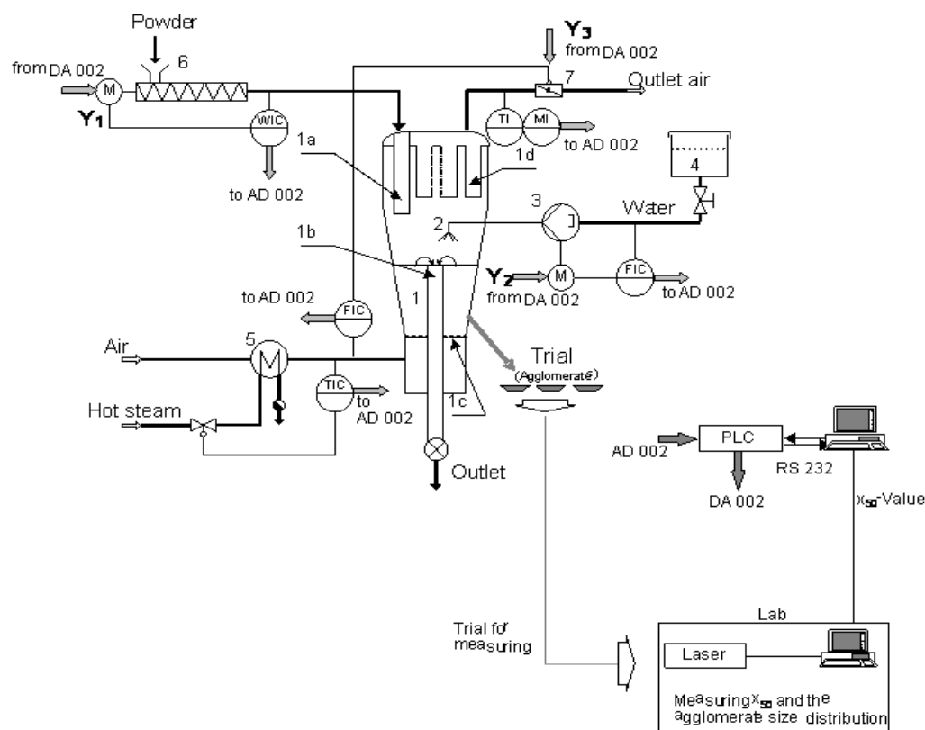
Figure 3. Experimental setup used for fluidized bed agglomeration: 1 – apparatus tower, 1a – down-pipe, 1b – stand-pipe, 1c – sieve, 1d – single-chamber shacking filter, 2 – spray nozzle, 3 – spray pump, 4 – spray solution, 5 – heater, 6 – differential dosing scale with a rotary valve, 7 – air outlet flap, Y_1 – powder mass flow (kg/h), Y_2 – fluid volume (ml/min), Y_3 – outlet air flap (%), AD002 – A/D converter, DA002 – D/A converter
