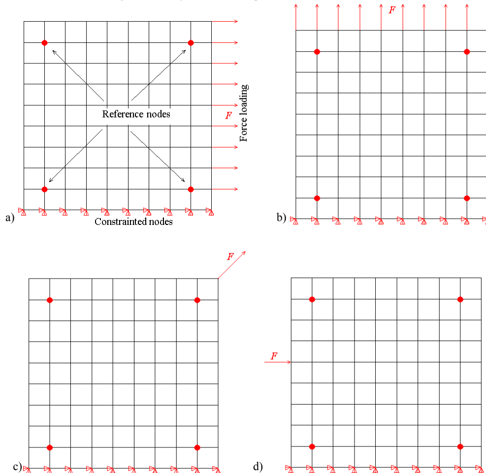
Figure 2. The finite element models: a) 1 st analysis model; b) 2 nd analysis model; c) 1 st test model; d) 2 nd test model
