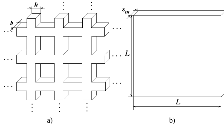
Figure 1. The girder (a) and equivalent steel membrane (b)
