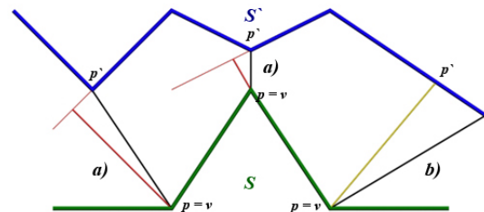
Figure 1. Two cases of the minimum distance: a) vertex-vertex; b) vertex-face
