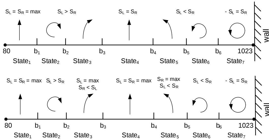
Figure 4. Schemes of intelligent state based control systems
