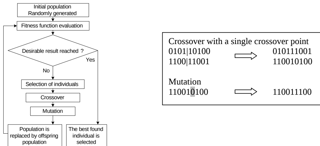
Figure 2. Scheme of Genetic Algorithm
