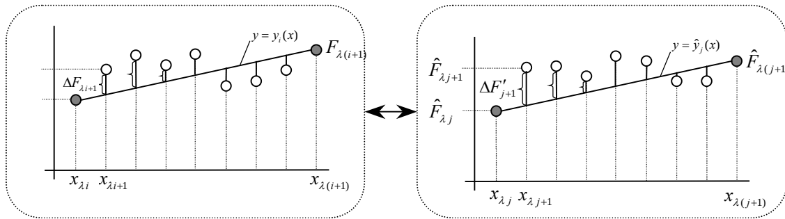
Figure 1. Organizing local collage for the set of real-data ( \lambda = 2^3 = 8 )
