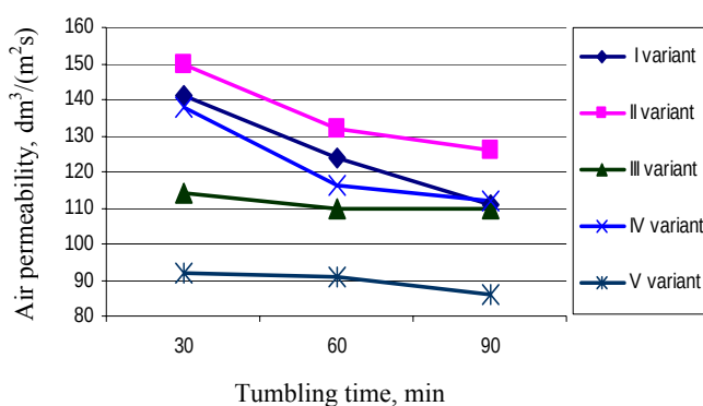
Fig. 7. Air permeability of the terry fabrics versus tumbling time
