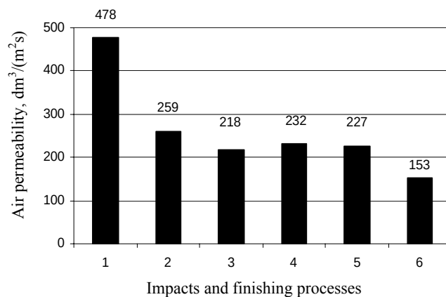
Fig. 1. Air permeability of terry fabrics with hemp pile regarding impacts and finishing process: 1 – without finishing (grey fabric); 2 – wetting; 3, 4, 5 – washing in 10, 30, 120 min without detergent; 6 – washing with detergent in 60 min
