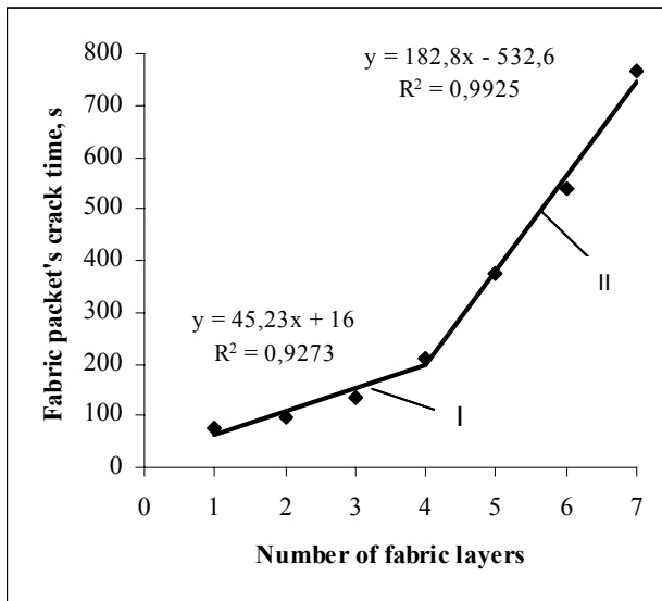
Fig. 3. Dependence of the fabric packet's crack time on number of fabric layers after dividing the burning process into two parts according the heat conduction theory
