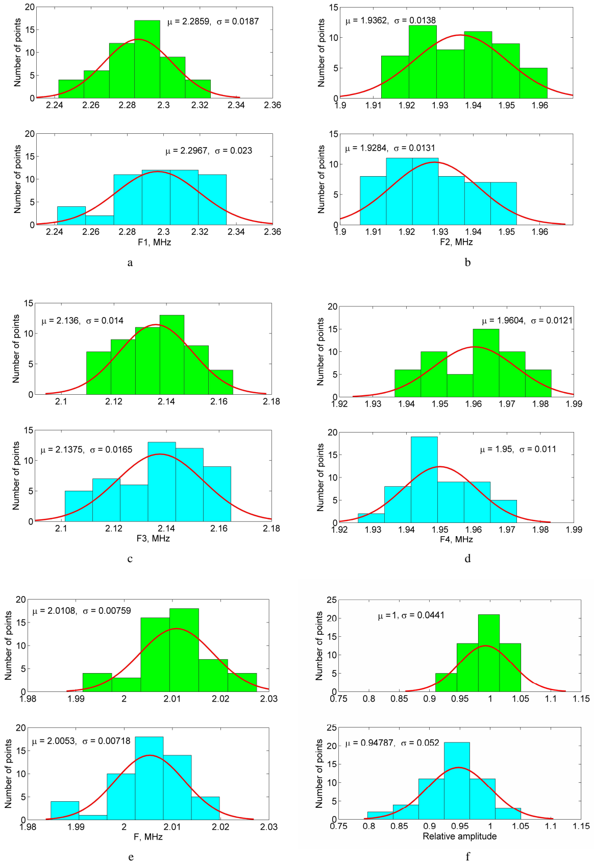
Fig. 3. Changes in transducer parameters affected by temperature shock tests: distribution changes of momentary frequencies F1 (a), F2 (b), F3 (c), F4 (d), central frequency F (e) and relative amplitude of the echo signal (f). (Parameters distributions before and after the tests are presented in upper and lower figures respectively)
