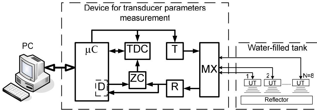
Fig. 2. Structural diagram of ultrasonic piezoelectric transducer testing equipment: \mu C – microcontroller, TDC – time-to-digital converter, T – transmitter, R – receiver, MX – multiplexer, UT – ultrasonic transducer, ZC – zero cross comparator, D – signal detector, PC – computer with application software
