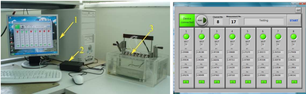
Fig. 1. Equipment for ultrasonic piezoelectric transducer testing: a) equipment photo, where 1 is PC, 2 is device for transducer parameters measurement, 3 is water-filled tank; b) is screenshot of the application software used for transducers' testing
