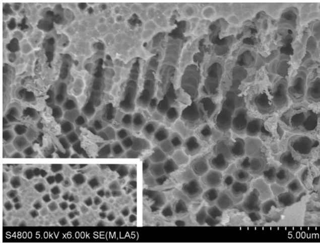
Fig. 2. Scanning electron microscope picture of porous silicon. The rectangle at the left bottom angle shows the 24.64 \mu\text{m}^2 area with 4.9 \mu\text{m}^2 pores area, which corresponds to the filling coefficient of 0.8
