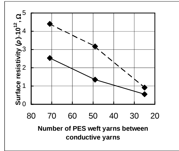
Fig. 3. Surface resistivity of the fabrics versus number of PES weft yarns between the conductive yarns ( — as received; - - - after 5 washing cycles) (Control fabric: as received \rho = 9.43 \times 10^{12} \Omega ; after 5 wash. cycles \rho = 9.98 \times 10^{13} \Omega )
