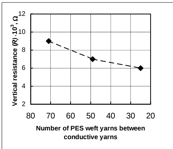
Fig. 4. Vertical resistance of the fabrics versus number of PES weft yarns between the conductive yarns: a – as received; (control fabric: R = 2.82 \times 10^{10} \Omega ); b – after 5 washing cycles (control fabric: R = 1.36 \times 10^{12} \Omega )
