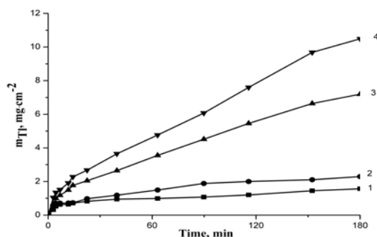
Fig. 7. Dependence of thallium content in sulphide layer on PE film on sulphurization time under treatment it with solution of \text{H}_2\text{S}_{33}\text{O}_6 at 60 °C for different periods of time. The sulphured PE treated with 0.1 M \text{Ti}_2\text{SO}_4 solution at 80 °C. Duration (min) of sulphured PE treatment with \text{Ti}_2\text{SO}_4 solution: 1–2, 2–5, 3–10, 4–20
