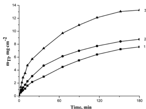
Fig. 6. Dependence of thallium content in sulphide layer on PE film on sulphurisation time under treatment it with solution of \text{H}_2\text{S}_{33}\text{O}_6 at 80 °C for different periods of time. The period of treatment with 0.1 M \text{Ti}_2\text{SO}_4 solution at 80 °C was 10 min. The concentration ( \text{mol}\cdot\text{dm}^{-3} ) of \text{Ti}_2\text{SO}_4 solution: 1–0.001, 2–0.05, 3–0.1
