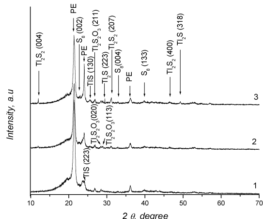
Fig. 8. X-ray diffraction patterns of thallium sulphide layers on the surface of PE. PE initially treated with a solution of \text{H}_2\text{S}_{33}\text{O}_6 at 60 °C for different times and then immersed in \text{Ti}_2\text{SO}_4 solution at 80 °C for 10 min. Sulphurization time (min): 1–15, 2–60, 3–120
