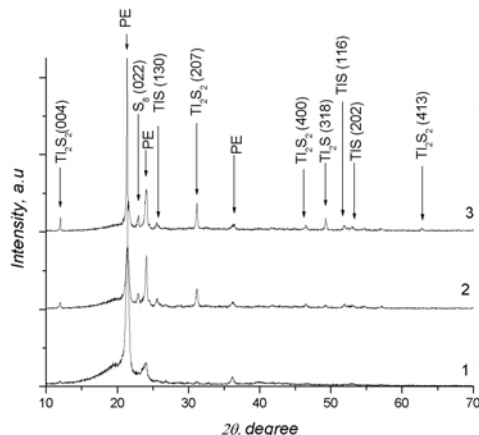
Fig. 9. X-ray diffraction patterns of thallium sulphide layers on the surface of PE. PE initially treated with a solution of \text{H}_2\text{S}_{33}\text{O}_6 at 80^\circ\text{C} for different times and then immersed in \text{Tl}_2\text{SO}_4 solution at 80^\circ\text{C} for 10 min. Sulphurisation time (min): 1–15, 2–60, 3–120
