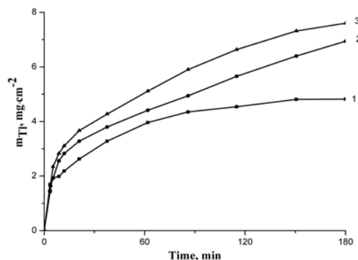
Fig. 5. Dependence of thallium content in sulphide layer on PE film on sulphurization time under treatment it with solution of \text{H}_2\text{S}_{33}\text{O}_6 at 60 °C for different periods of time. The period of treatment with 0.1 M \text{TI}_2\text{SO}_4 solution at 80 °C was 10 min. The concentration ( \text{mol}\cdot\text{dm}^{-3} ) of \text{TI}_2\text{SO}_4 solution: 1–0.001, 2–0.05, 3–0.1
