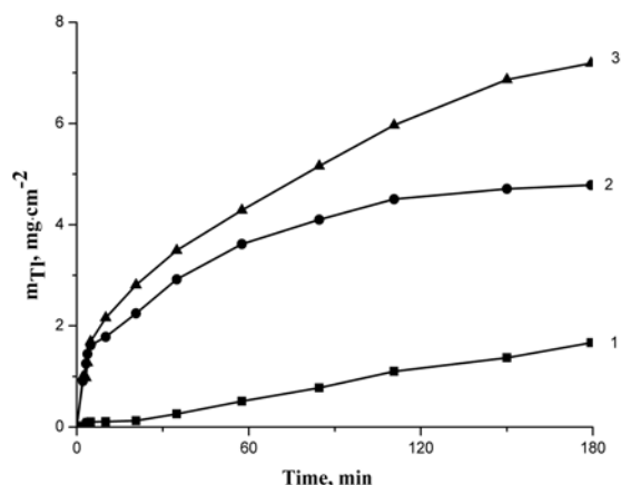
Fig. 4. Dependence of thallium content in sulphide layer on PE film on sulphurization time under treatment it with solution of \text{H}_2\text{S}_{33}\text{O}_6 at 60 °C for different periods of time. The period of treatment with 0.1 M \text{TI}_2\text{SO}_4 solution was 10 min. The temperature (°C) of \text{TI}_2\text{SO}_4 solution: 1–40, 2–60, 3–80
