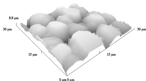
Fig. 11. AFM image of \text{Tl}_x\text{S}_y films on polyethylene. PE initially treated with a solution of \text{H}_2\text{S}_{33}\text{O}_6 at 60^\circ\text{C} for 120 min and then immersed in \text{Tl}_2\text{SO}_4 solution at 80^\circ\text{C} for 10 min
