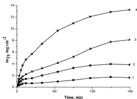
Fig. 3. Dependence of the content of thallium in sulphide layer on PE film on sulphurization time under treatment it with solutions of \text{H}_2\text{S}_{33}\text{O}_6 for different periods of time. The period of treatment with 0.1 M \text{TI}_2\text{SO}_4 solution at 80 °C was 10 min. The temperature (°C) of \text{H}_2\text{S}_{33}\text{O}_6 solution: 1–25, 2–40, 3–60, 4–80
