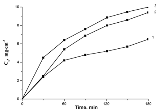
Fig. 1. Dependence of the content of sulphur in layer on PE film on sulphurization time under treatment it with solutions of H _2 S _n O _6 at 60 °C. The average number of sulphur number atoms ( n ) in polythionic acid molecule: 1–21; 2–33; 3–45
