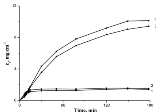
Fig. 2. Dependence of the content of sulphur in layer on PE film on sulphurization time under treatment it with solutions of H _2 S _{33} O _6 . The temperature (°C) of H _2 S _{33} O _6 solution: 1–25, 2–40, 3–60, 4–80
