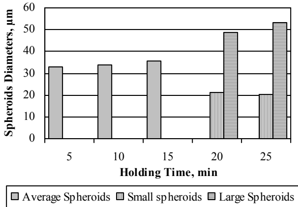
Fig. 3. Size of the graphite spheroids diameters in 10 mm thick plates as a function of the time after spheroidizing treatment
