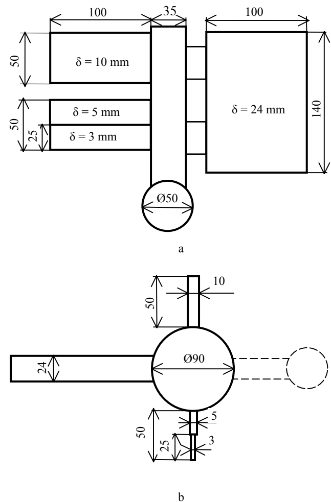
Fig. 1. Horizontal (a) and vertical (b) test castings (dimensions in millimetres)
