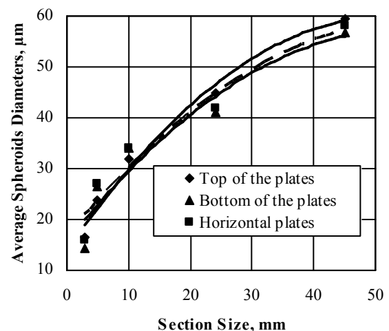
Fig. 2. Effect of the sections size of the vertical and horizontal specimens on the diameter of the graphite spheroids
