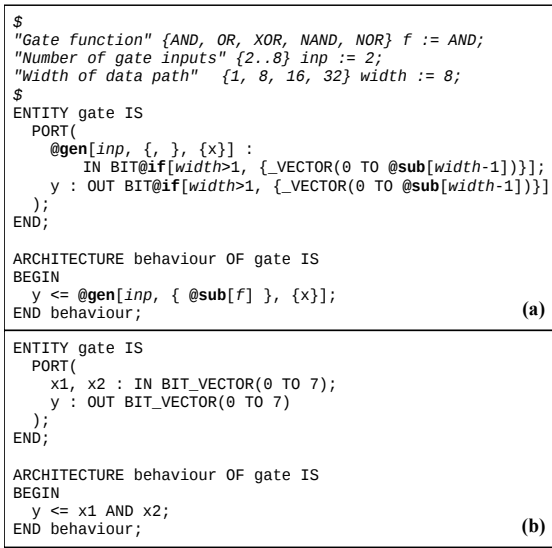
Figure 2. Example of the concepts of metaprogramming
