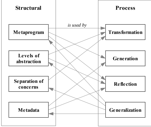
Figure 1. Relationship between structural and process concepts of metaprogramming
