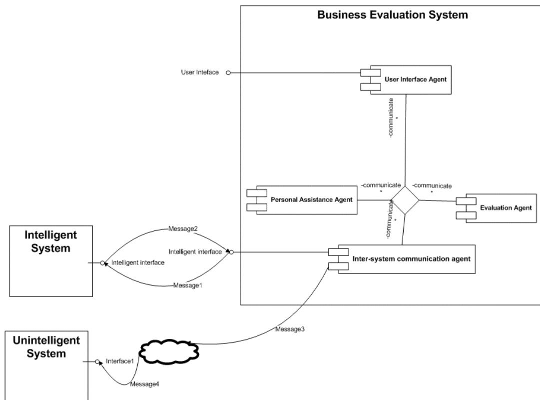
Figure 3. Architecture of Business Evaluation System
