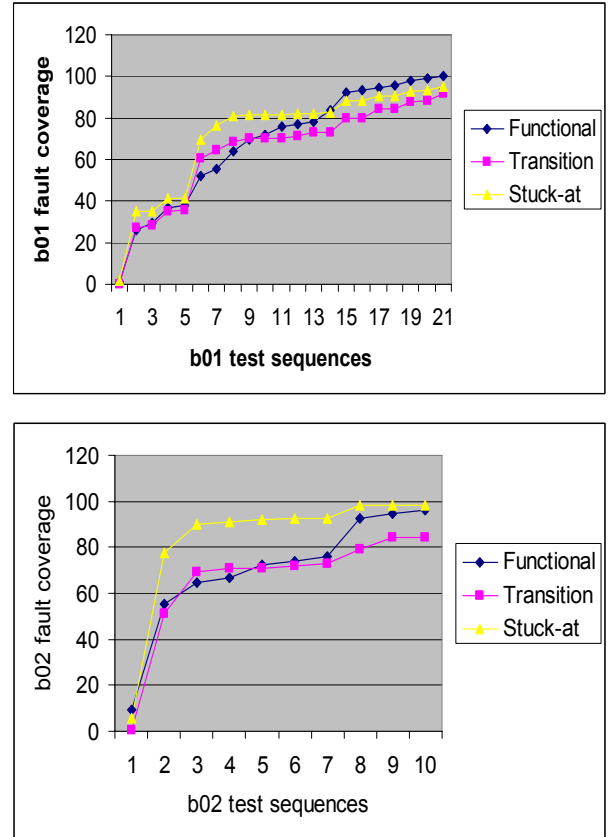
Figure 1. The process of covering faults of benchmarks b01 and b02
