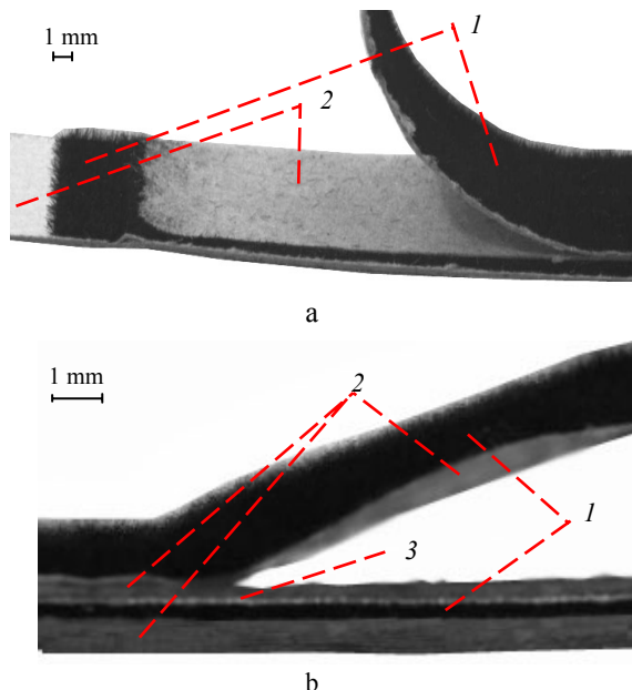
Fig. 4. Photo of a glued (glue Eukalin) flocked sample made from 1 mm-length Capron flock and paperboard Duoplex UD-3, after breaking off: a – view from the top; b – section view; 1 – flock coating; 2 – paperboard; 3 – glue layer
