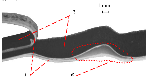
Fig. 7. Photo of a glued (glue Eukalin) flocked sample made from 1 mm-length Capron flock and paperboard Alaska GC-2, after breaking off: 1 – paperboard; 2 – flock coating; e – inner delamination
