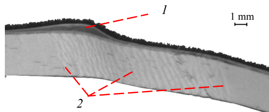
Fig. 8. Photo of a glued (glue Eukalin) flocked sample made from 1 mm-length Capron flock and paperboard Arktika GC-1, after breaking off: 1 – inner delamination; 2 – warping
