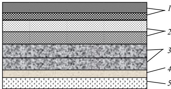
Fig. 1. Structure of elementary paperboard layers: 1 – chalk-coated layers (up to 3 layers); 2 – top layer (face side) – one or several layers of good quality raw material (bleached or unbleached cellulose, wood pulp, bleached paper waste); 3 – insert (combination of middle paperboard layers) – quite a thick layer from cheap raw material – paper waste, wood pulp, unbleached cellulose; 4 – bottom layer – one or several layers of good quality raw material; 5 – surface sizing
