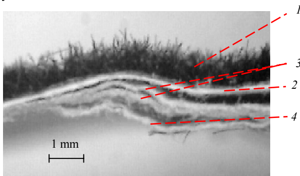
Fig. 2. Photo of the structure of a flocked printing sample: 1 – flock coating; 2 – top paperboard layer; 3 – insert; 4 – bottom paperboard layer
