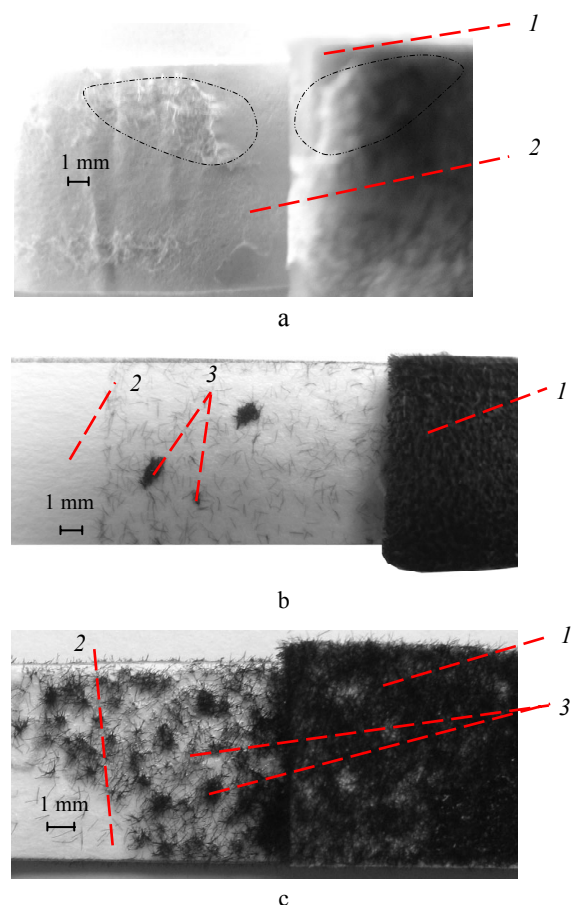
Fig. 3. Photo of the glued (glue Eukalin) flocked samples with a flock coating on paperboard: Arktika GC-1 after breaking off: a – 0.5 mm-length Capron; b – 0.75 mm-length viscose; c – 1.0 mm-length Capron: 1 – flock-coating (face side); 2 – paperboard (reverse side of flocked packaging); 3 – broken-off flock fibres
