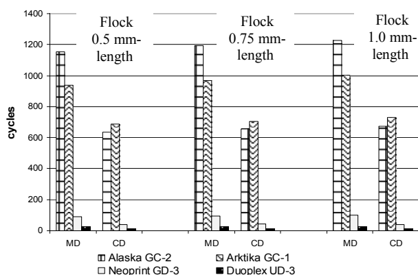
Fig. 11. Number of double folds of flock printing materials depending on the paperboard type and size of flock
