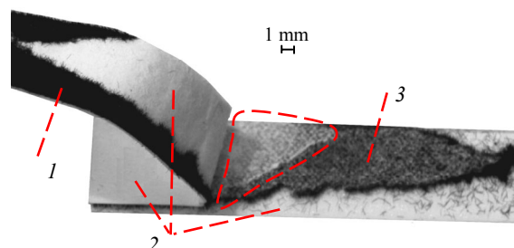
Fig. 5. Photo of a glued (glue Eukalin) flocked sample made from 1 mm-length Capron flock and paperboard Arktika GC-1, after breaking off: 1 – flock coating; 2 – paperboard; 3 – broken off flock coating
