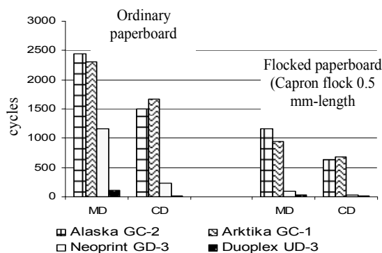
Fig. 10. Number of double folds depending on the paperboard type
