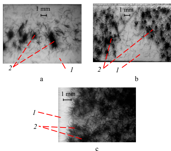
Fig. 6. Photo of glued (glue Eukalin) flocked samples (view from above) made from 1 mm-length Capron flock on paperboard Arktika GC-1 after breaking off: 1 – paperboard; 2 – broken off flock fibers
