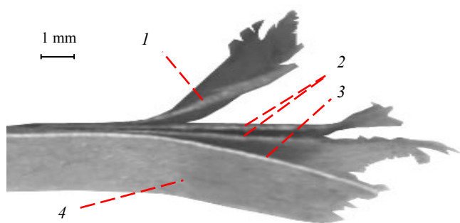
Fig. 9. Photo of flocked sample made from 0.5 mm-length Capron flock and paperboard Duoplex UD-3, when testing the number of double-folds: 1 – bottom layer of the paperboard; 2 – insert; 3 – top layer; 4 – flock coating
