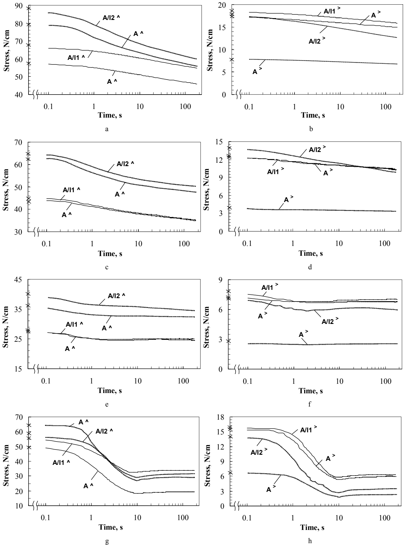
Fig. 3. Stress relaxation of fabric A and fused systems A/I1 and A/I2 (a, b) and when the specimens are being stretched after hygrothermal treatment (c, d); when specimens are being steaming during the stretching process (e, f); when specimens are being steaming after the stretching process (g, h): ^ – lengthwise; > – crosswise; — – when lengthwise \varepsilon = 9\% , crosswise \varepsilon = 8\% ; ..... – when lengthwise \varepsilon = 14\% , crosswise \varepsilon = 6\% ; × – initial stress value
