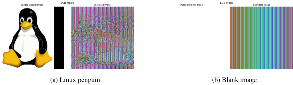
Fig. 14. ECB Mode of our cipher with \mathbb{GF}(2^9) platform group applied to monochromatic image.
