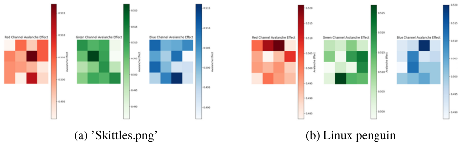
Fig. 19. Heatmaps for the avalanche criterion of our cipher with \text{GF}(2^9) platform group.
