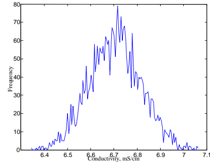
Fig. 5. Distribution of milk conductivity measurement results
