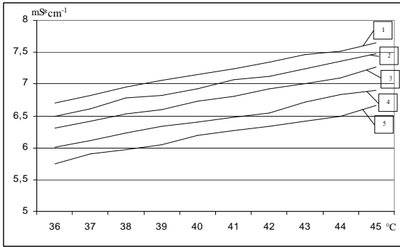
Fig. 1. Dependence of milk conductivity and temperature of the sample
