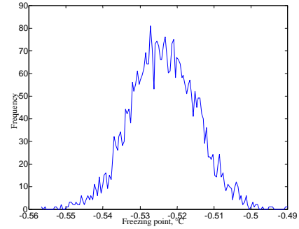
Fig. 6. Distribution of milk freezing point measurement results
