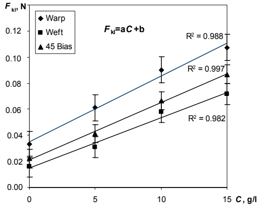
Fig. 5. Dependence of buckling force F_{kl} on stiffener concentration C
