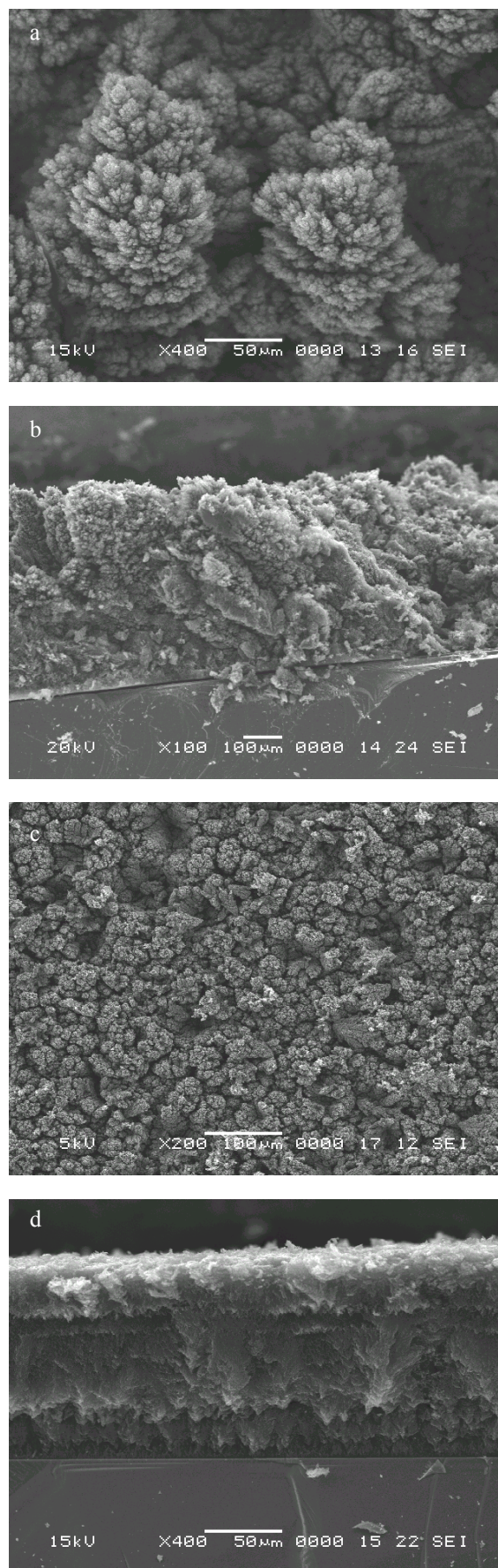
Fig. 1. SEM surface morphology (a, c) and cross-section (b, d) of carbon films deposited at various \text{Ar/C}_2\text{H}_2 ratios: a, b – \text{Ar/C}_2\text{H}_2 = 12:1 ; c, d – \text{Ar/C}_2\text{H}_2 = 100:1
