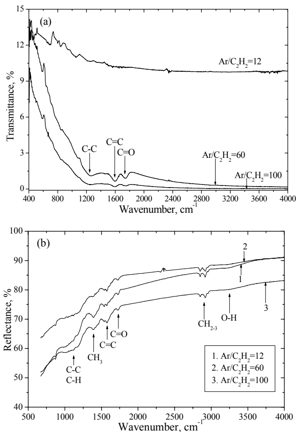
Fig. 2. FTIR transmittance (a) and reflectance (b) spectra of the carbon coatings formed at different \text{Ar}/\text{C}_2\text{H}_2 ratios
