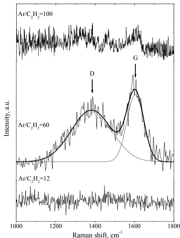
Fig. 3. Raman spectra of carbon coatings formed at various \text{Ar}/\text{C}_2\text{H}_2 ratios
