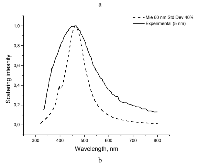
Fig. 6. Spectra of Ag spherical particles in PMMA matrix at different thickness of Ag film: a – 1 nm and b – 5 nm
