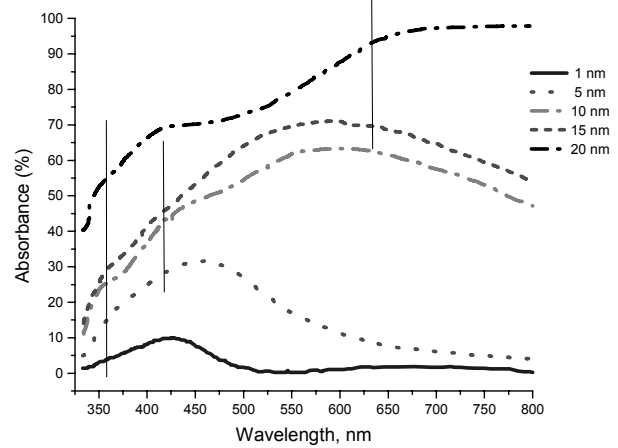
Fig. 5. Absorbance spectra of Ag-PMMA-PET structure
