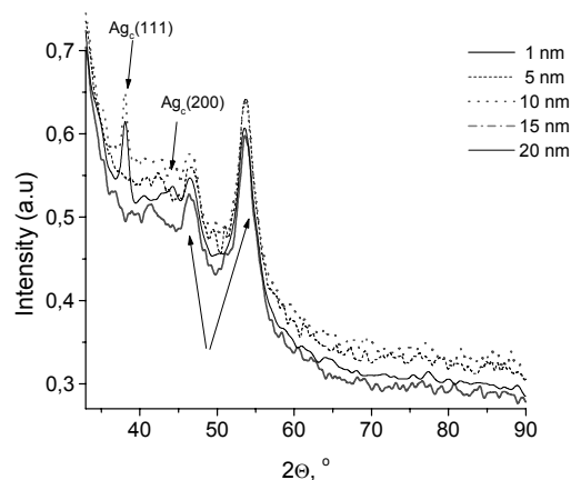
Fig. 2. XRD pattern of Ag films on PMMA-PET substrate of different thickness
