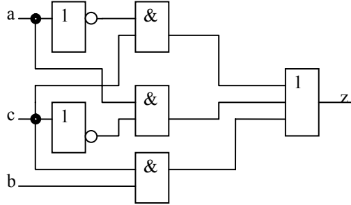
Figure 1. A realization of function z = ac' + a'c + bc
