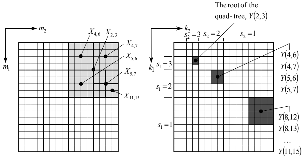
Figure 3. Graphical interpretation of properties of Haar spectral coefficients: (a) image [X(m_1, m_2)] , N=16 ; the coefficient Y(2, 3) is associated with the image block X_{2,3} ; (b) the quad-tree, attached to the Haar coefficient Y(2, 3) ( \mathfrak{I}_2 = \{4, 5, 8, 9, 10, 11\} , \mathfrak{I}_3 = \{6, 7, 12, 13, 14, 15\} )
