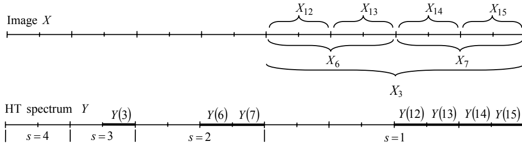
Figure 2. Graphical interpretation of properties of Haar spectral coefficients ( \mathfrak{I}_3 = \{6, 7, 12, 13, 14, 15\} represents the tree, attached to the spectral coefficient (root of the tree) Y(3) ; N=16 )
