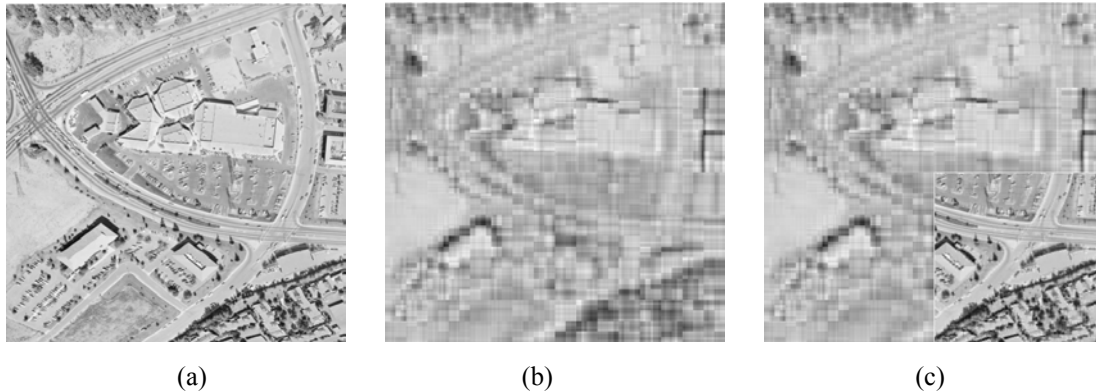
Figure 6. Locally progressive encoding of test images: (a) original image survey.bmp 512x512; (b) the rough estimate of the whole image ( \beta_1 = 35 ); (c) the selected image fragment of size 256x256 compressed at a ratio \beta_2 = 3
