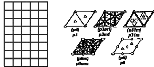
Fig. 5. Symmetry groups unrealizable for non-Jacquard woven ornaments
