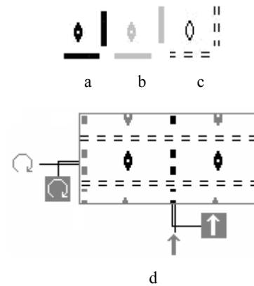
Fig. 7. Main principles of new notation system: a – active axes and centres, b – dependent elements, c – elements having indispensable position, d – example of ornament representation
