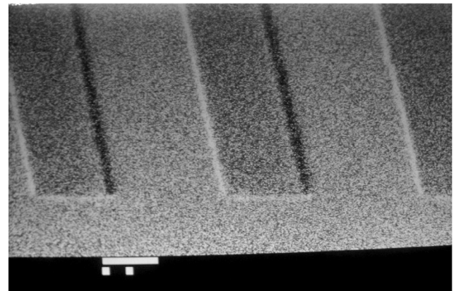
Fig. 2. SEM view of the imprinted resist film with SiO_x – doped DLC film mould. Mark size 10 μm
