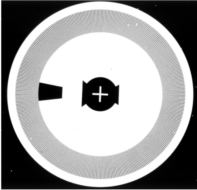
Fig. 1. Optical microscope view of the silicon imprint mould of the angular encoder (dimensions of the central cross are 0.5×0.5 mm, the width of the cross line is 20 μm), and detail of the scale (length of lines is 0.75 mm, scale pitch in the center of lines is 20 μm)
