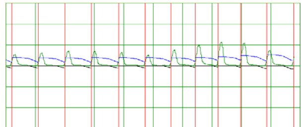
Fig. 6. Beat detection with adaptive thresholds
