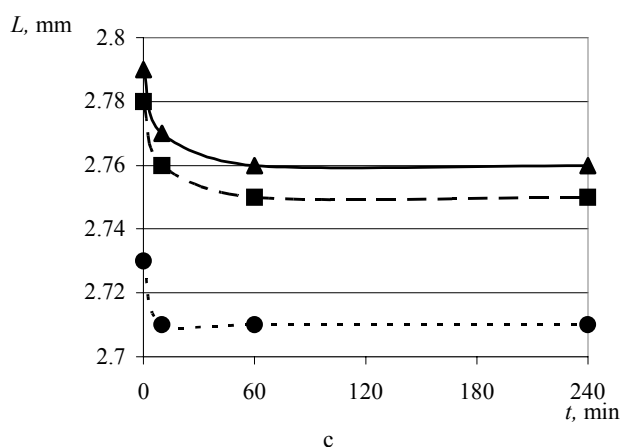
Fig. 2. Dependence of plain weave fabric the stitch length L(x) upon internal friction ( \text{tg}\delta ) and time t , when rotational frequency of the main shaft is the following: a – 200 \text{ min}^{-1} , b – 1100 \text{ min}^{-1} , c) 2100 \text{ min}^{-1} (---- 0.03, — 0.033, ---- 0.037)
