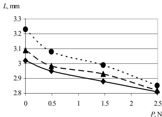
Fig. 5. Dependence of the stitch length L upon two-sided load P and rotational frequency of the main shaft, when pressing force is 45 N and external friction force of fabric is 10.9 N (— — 200 \text{min}^{-1} , --- — 1100 \text{min}^{-1} , ..... — 2100 \text{min}^{-1} )
