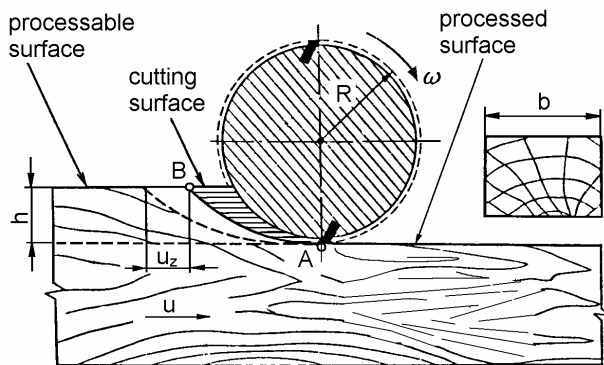
Fig. 1. Technological scheme of longitudinal milling [1]
