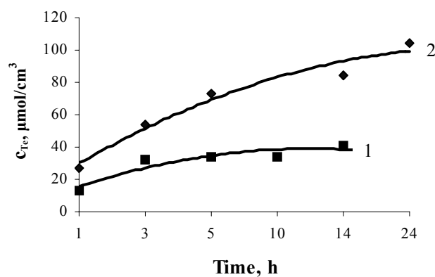
Fig. 3. Change of tellurium concentration in PA with time during its treatment with a \text{H}_2\text{TeS}_4\text{O}_6 solution at 20 °C. The concentration of \text{H}_2\text{TeS}_4\text{O}_6 solution, \text{mol}\cdot\text{dm}^{-3} : 1 – 0.01, 2 – 0.05
