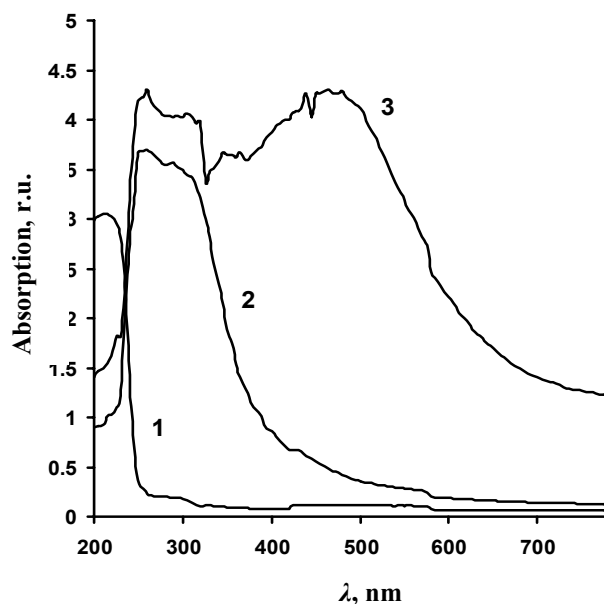
Fig. 2. UV absorption spectra: 1 – of PA film, 2 – of PA surface after 24 h exposure in 0.1 \text{ mol}\cdot\text{dm}^{-3} solution of \text{H}_2\text{TeS}_4\text{O}_6 at 20 °C, 3 – of copper chalcogenides on PA after interaction with \text{Cu}(\text{II/I}) salt solution
