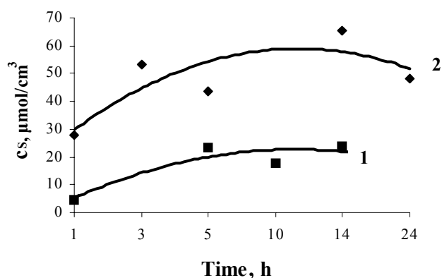
Fig. 4. Change of sulfur concentration in PA with time during its treatment with a \text{H}_2\text{TeS}_4\text{O}_6 solution at 20 °C. The concentration of \text{H}_2\text{TeS}_4\text{O}_6 solution, \text{mol}\cdot\text{dm}^{-3} : 1 – 0.01, 2 – 0.05
