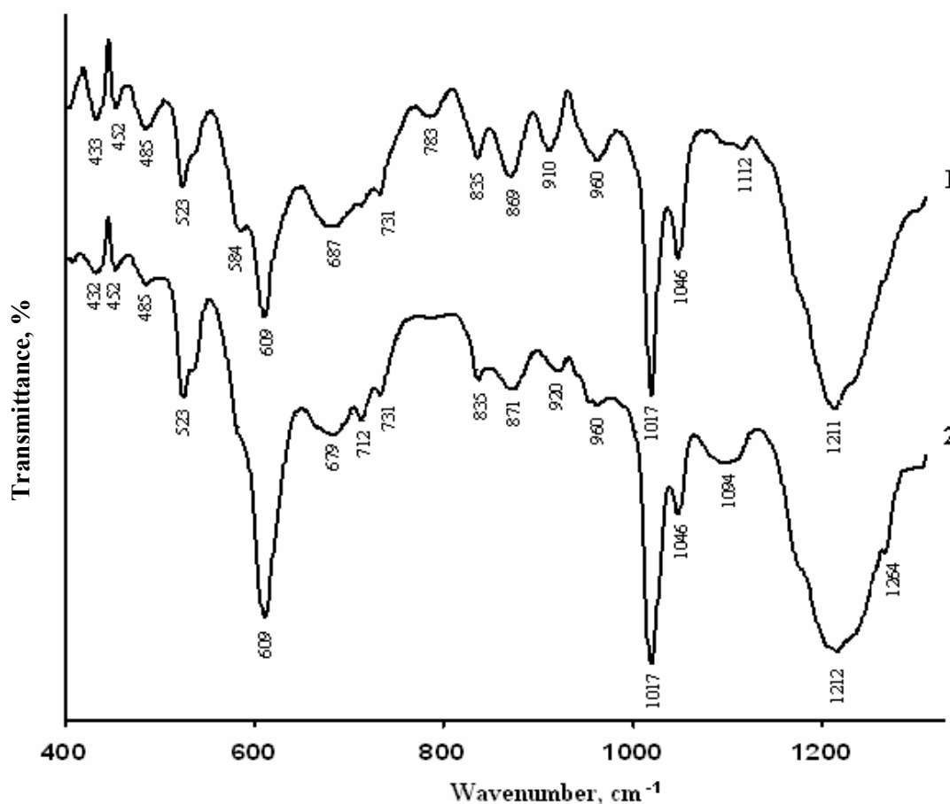
Fig. 1. IR absorption spectra of a PA films treated with a solution of \text{H}_2\text{TeS}_4\text{O}_6 of different concentration at 20 °C during 121 h. The concentration of \text{H}_2\text{TeS}_4\text{O}_6 solution, \text{mol}\cdot\text{dm}^{-3} : 1 – 0.01, 2 – 0.05
