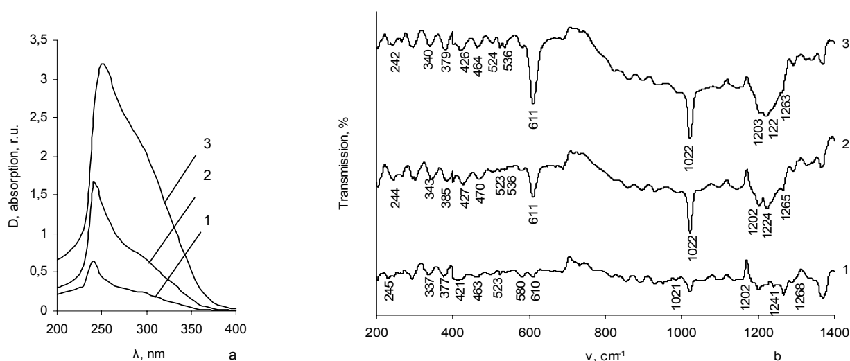
Fig. 2. UV (a) and IR (b) absorption spectra of PKA films sulfured in 0.15 \text{ mol} \cdot \text{dm}^{-3} \text{ K}_2\text{S}_5\text{O}_6 solution in 0.1 \text{ mol} \cdot \text{dm}^{-3} \text{ HCl} (pH 1.5) at time of 4 h of different temperature. The temperature of PKA sulfuration, ^\circ \text{C} : 1 – 0; 2 – 10; 3 – 20
