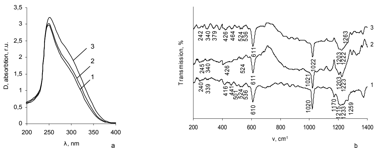
Fig. 1. UV (a) and IR (b) absorption spectra of PKA films sulfured in 0.15 \text{ mol} \cdot \text{dm}^{-3} \text{ K}_2\text{S}_5\text{O}_6 solution in 0.1 \text{ mol} \cdot \text{dm}^{-3} \text{ HCl} (pH 1.5) at 20^\circ \text{C} temperature of different time. Time of duration, h: 1 – 2; 2 – 3; 3 – 4
