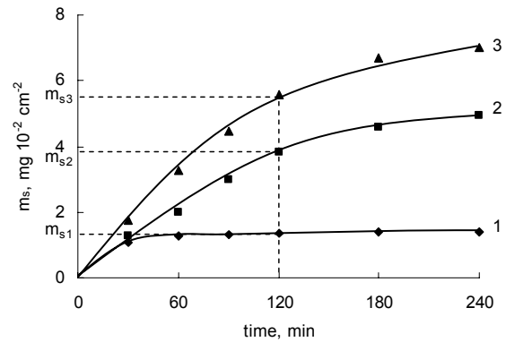
Fig. 4. The dependence of adsorbed sulfur amount in polycapraamide on exposure time in solution of \text{K}_2\text{S}_5\text{O}_6 ( c = 0.15\text{ mol}\cdot\text{dm}^{-3} ) at temperatures. Temperature, ^\circ\text{C} : 1 – 0; 2 – 10; 3 – 20
