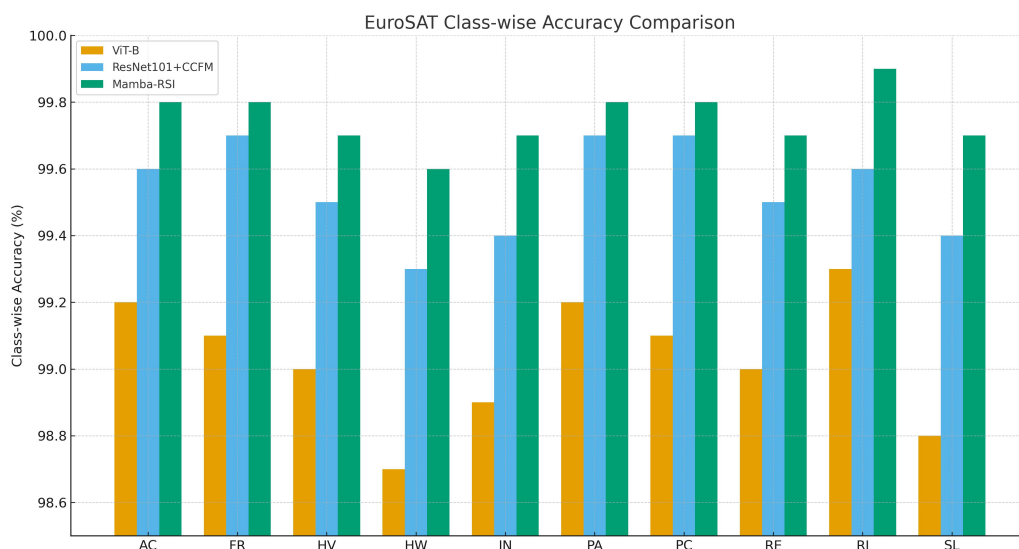
Figure 9. Class-wise classification accuracy comparison on the EuroSAT dataset across ViT-B, ResNet101+CCFM, and the Mamba-RSI model.
