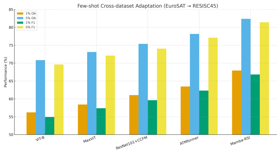
Figure 16. Few-shot cross-dataset adaptation performance for models trained on EuroSAT and fine-tuned on NWPU-RESISC45 using 1% and 5% labeled target samples, reported for OA and F1.
