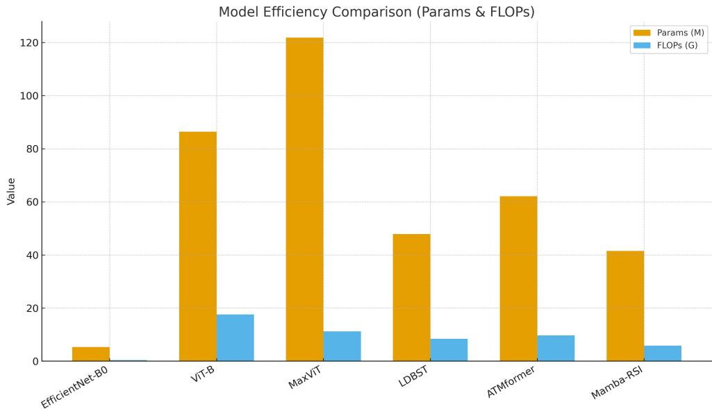
Figure 14. Comparison of model efficiency in terms of parameter count and computational complexity (FLOPs) for 224 \times 224 input resolution across state-of-the-art baselines and the Mamba-RSI framework.
