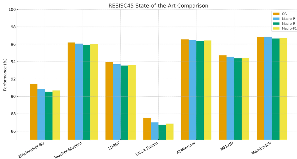
Figure 13. State-of-the-art comparison on the NWPU-RESISC45 dataset across overall accuracy, macro-precision, macro-recall, and macro-F1.
