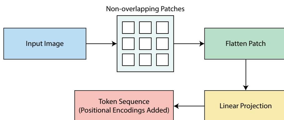
Figure 2. Patch embedding and tokenization process in Mamba-RSI.
