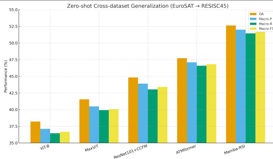
Figure 15. Zero-shot cross-dataset generalization performance for models trained on EuroSAT and directly evaluated on the NWPU-RESISC45 dataset without fine-tuning, reported across OA, macro-precision, macro-recall, and macro-F1.
