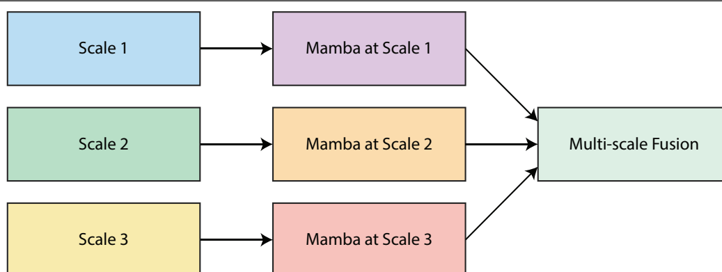
Figure 4. Hierarchical multi-scale feature extraction in Mamba-RSI.
