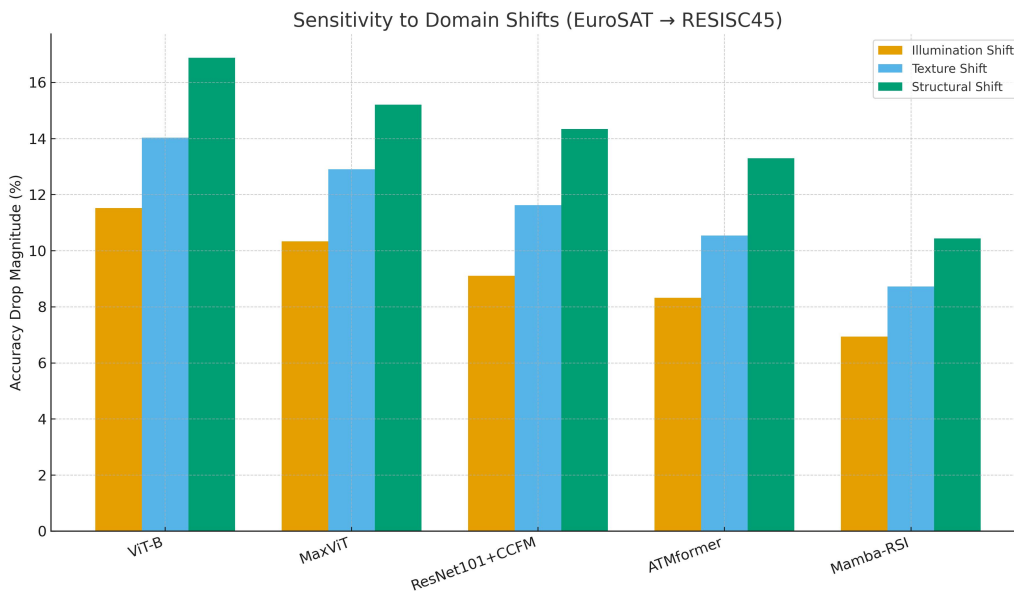
Figure 17. Sensitivity to domain shifts during cross-dataset transfer from EuroSAT to NWPU-RESISC45, measured as accuracy drop under illumination, texture, and structural perturbations.
