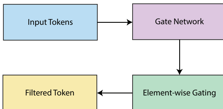
Figure 5. Selective gating mechanism used in the Mamba encoder.
