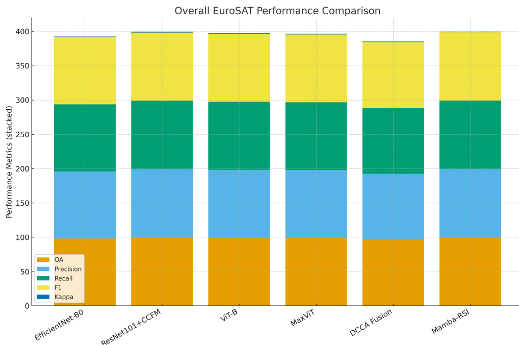
Figure 8. Comparison of overall classification performance on the EuroSAT dataset across competing models in terms of OA, precision, recall, F1-score, and the kappa coefficient.
