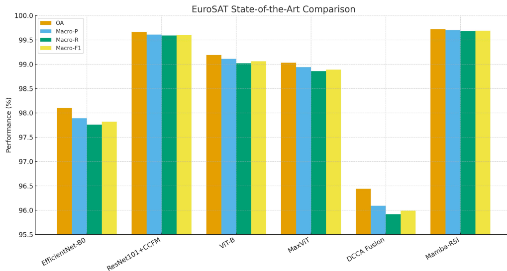
Figure 12. State-of-the-art comparison on the EuroSAT dataset across overall accuracy, macro-precision, macro-recall, and macro-F1.
