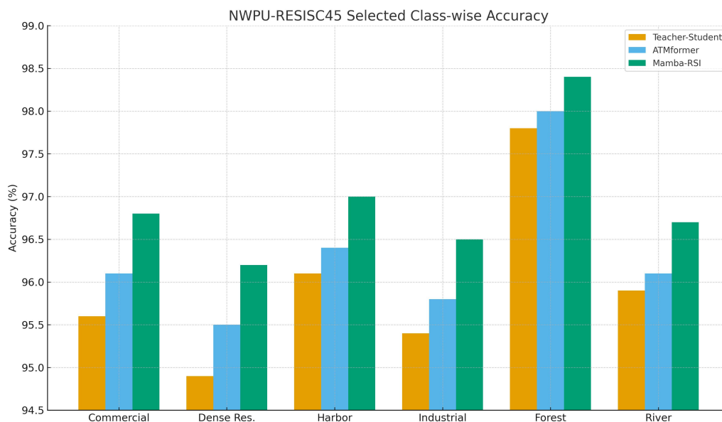
Figure 11. Selected class-wise classification accuracy comparison on the NWPU-RESISC45 dataset across teacher–student distillation, ATMformer, and the Mamba-RSI framework.
