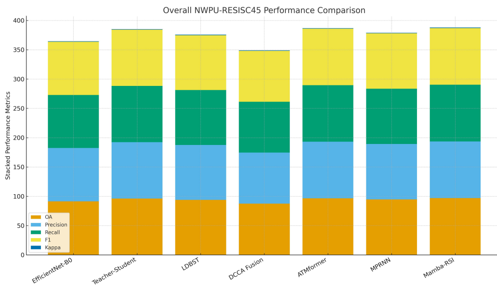
Figure 10. Comparison of overall classification performance on the NWPU-RESISC45 dataset in terms of OA, precision, recall, F1-score, and the kappa coefficient across all evaluated models.
