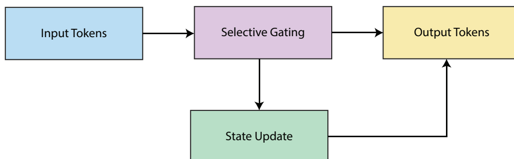
Figure 3. Schematic of a single Mamba state-space encoder block.
