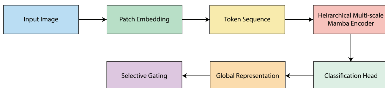
Figure 1. Overall architecture of the Mamba-RSI framework for land-use and land-cover classification.
