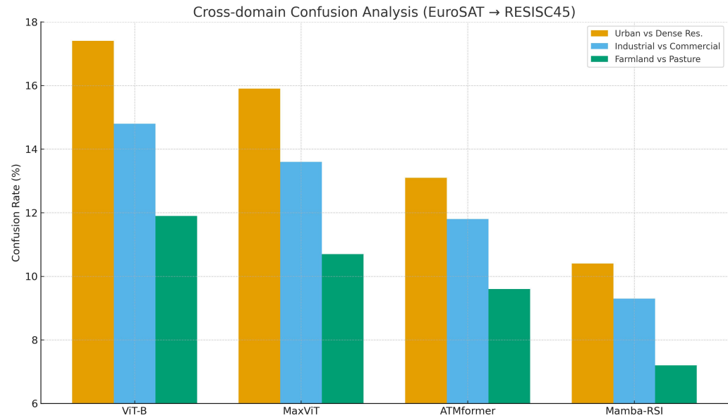
Figure 18. Cross-domain confusion analysis for visually similar scene pairs when transferring from EuroSAT to NWPU-RESISC45, reported as misclassification percentages across competing models.
